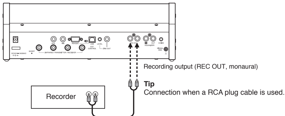
Central unit TS-820RC/820 (Rear panel)
