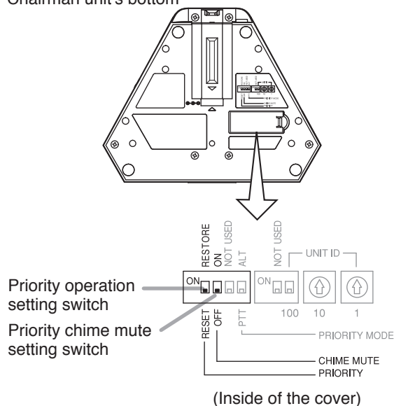
Chairman unit's bottom
